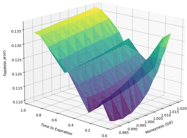
Figure 1: Local Volatility Surface.
